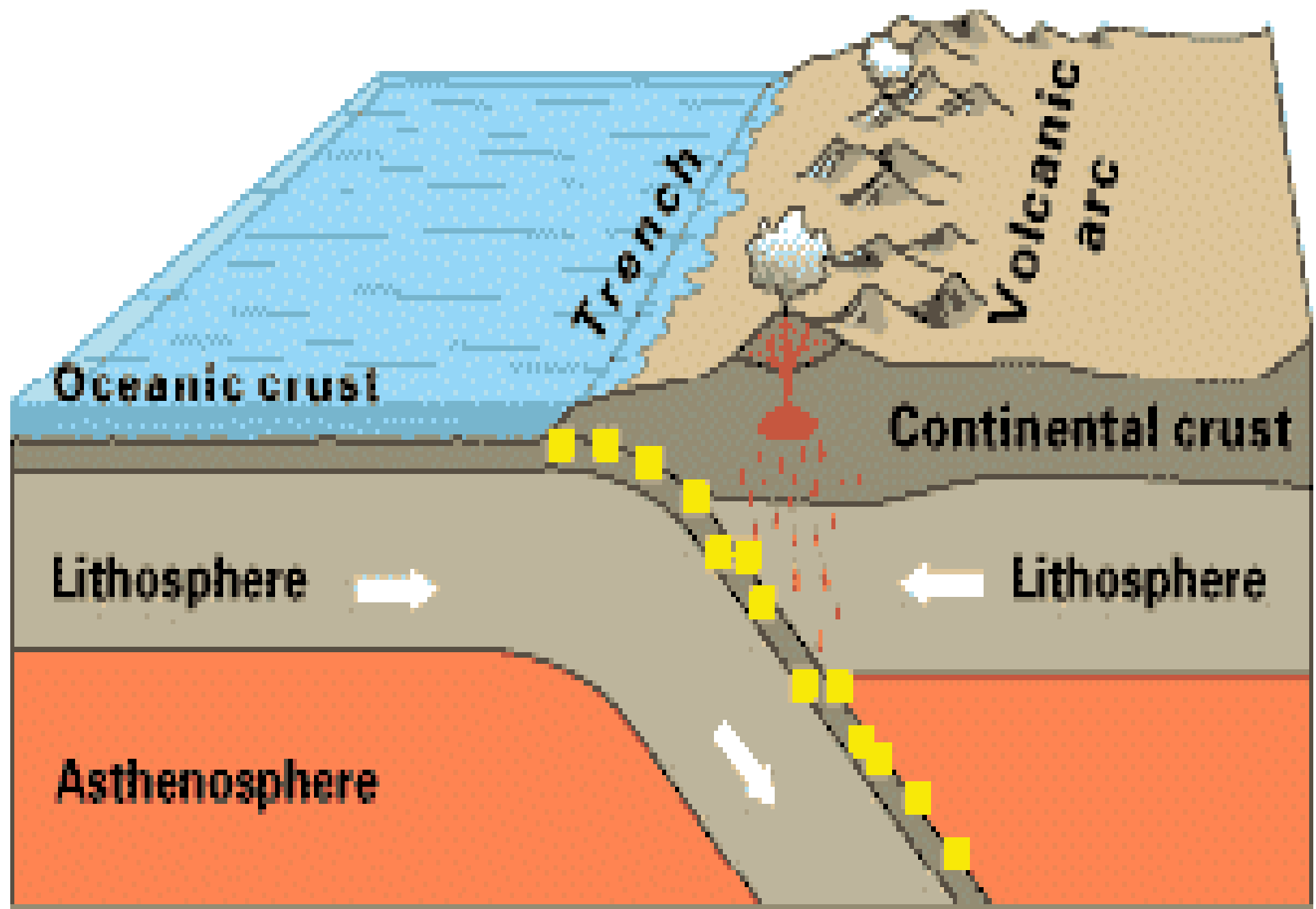
Oceanic-continental convergence
